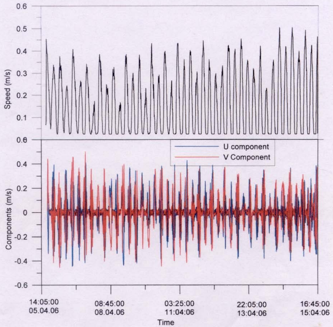
Figure 4.2.4: Current speed and components at station 2 during April 2006.
