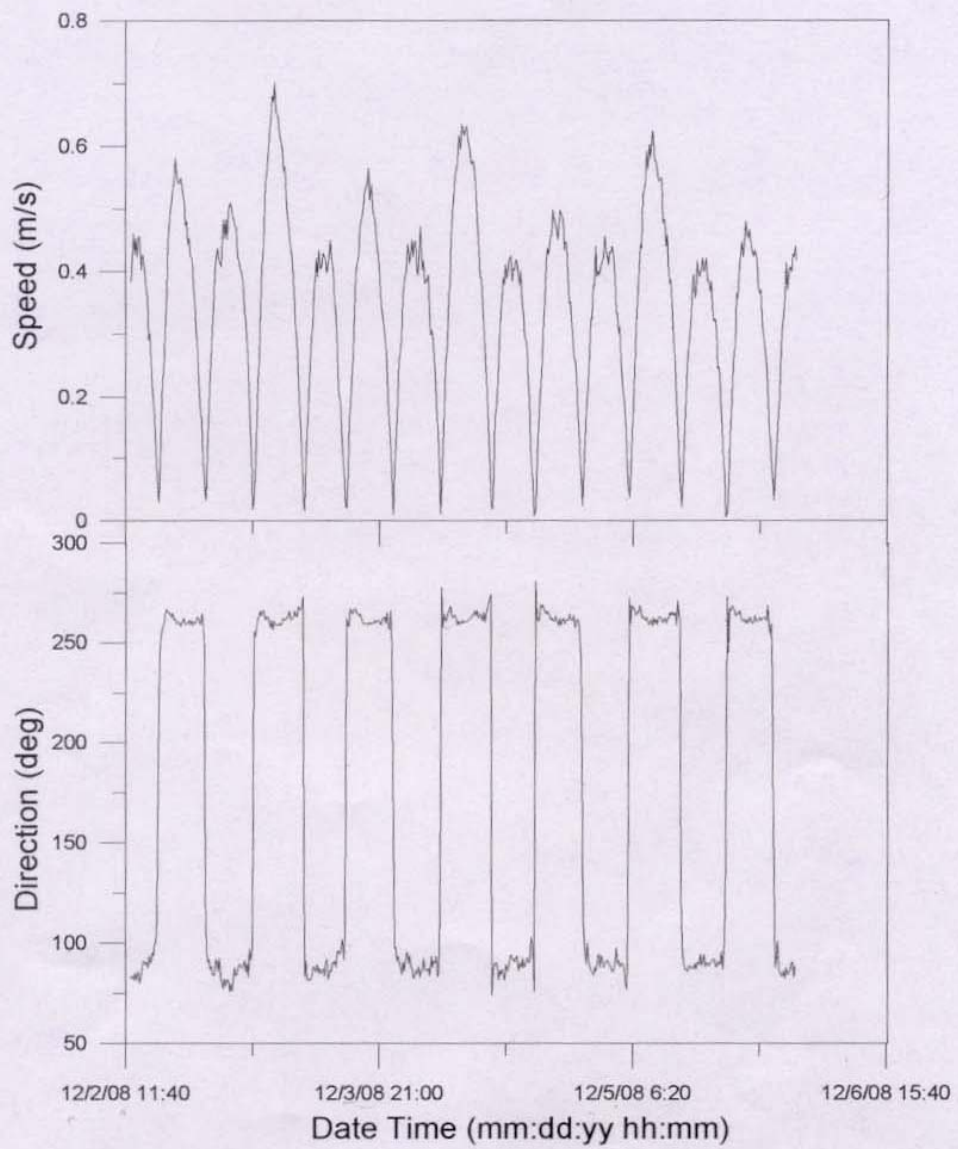
Figure 4.2.5: Current speed and direction at station 2 during December 2008.
