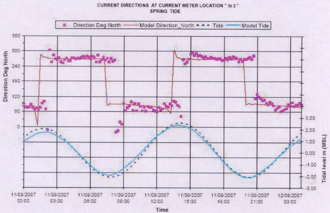
Figure 6.1.1: Comparison of simulation and observed currents at Station 2 (Spring)
