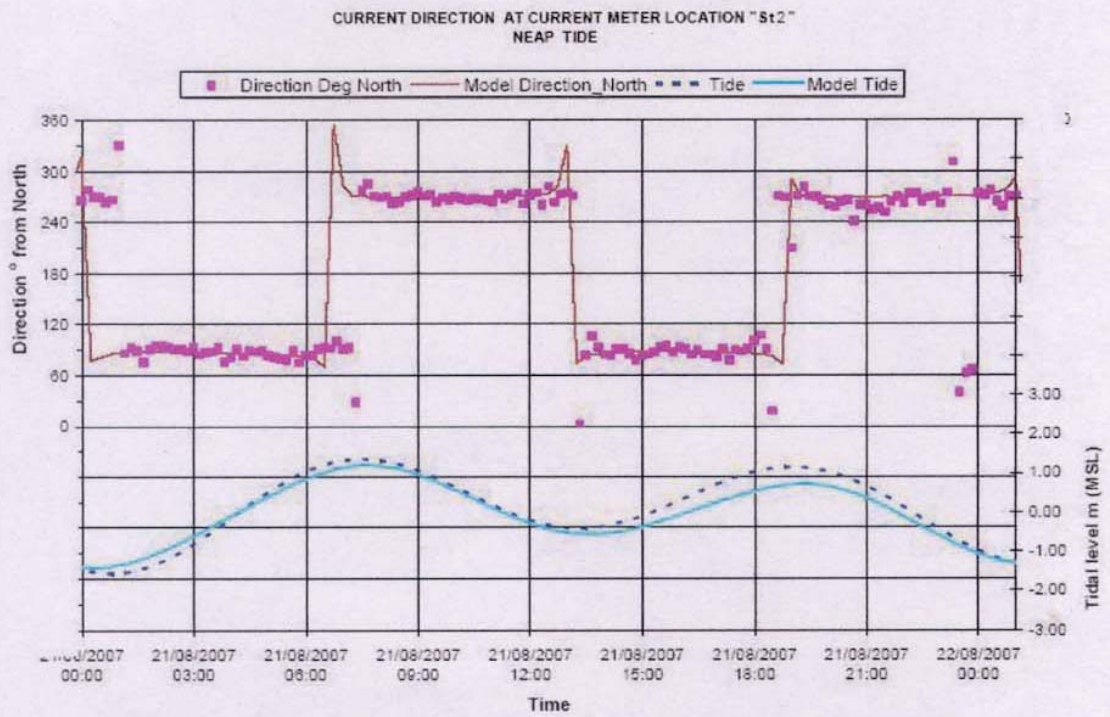
Figure 6.1.2: Comparison of simulation and observed currents at Station 2 (Neap)
