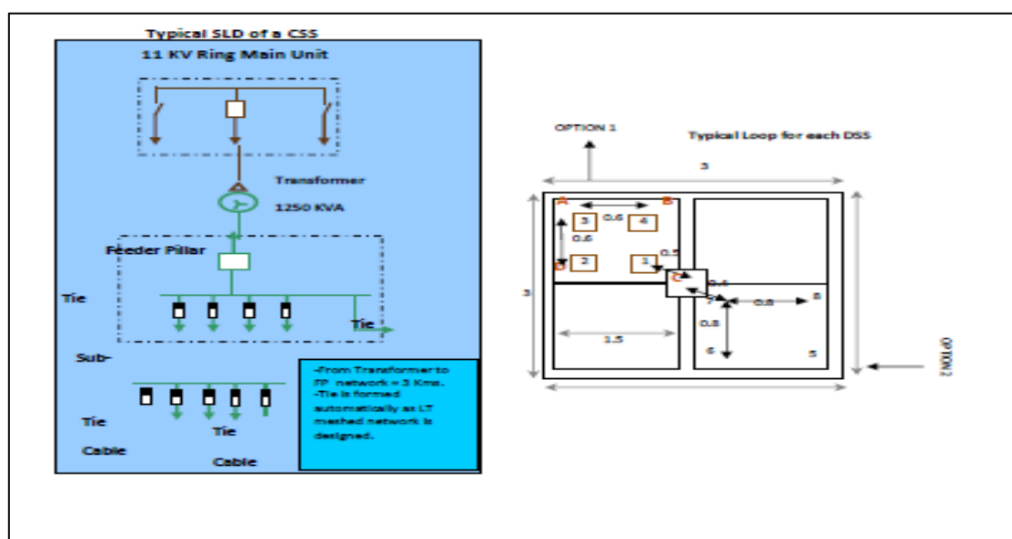
Figure 3: Typical arrangement of CSS
