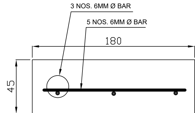
SECTION B-B
