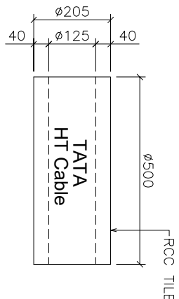
PLAN FOR HALF CIRCULAR RCC TILE
