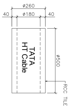
PLAN FOR HALF CIRCULAR RCC TILE
