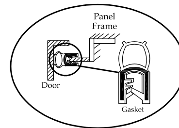
Detail's 'A'
