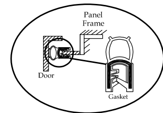
Detail's 'A'
