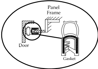
Detail's 'A'
